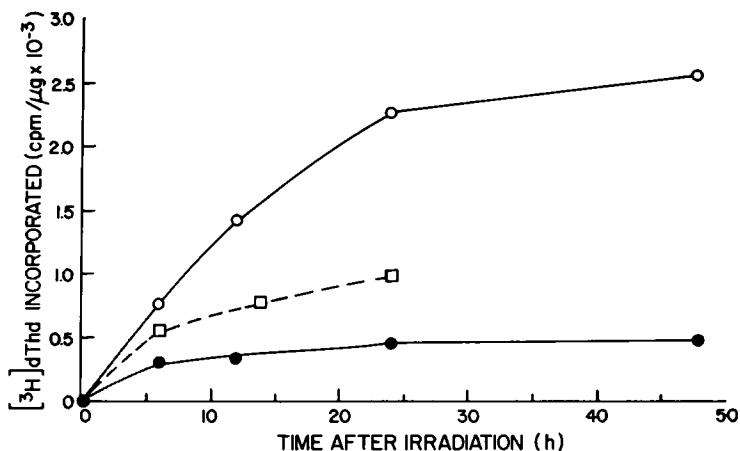
FIGURE 2 Rate of incorporation of [ ^3\text{H} ]-dThd into parental DNA by repair replication. Cells were plated into dishes, grown to confluence, irradiated with 40 J/m 2 (O), 15 J/m 2 (□), or 7 J/m 2 (●) of UV radiation, and incubated for the indicated time periods in labeling medium. The DNA was extracted, and incorporation of [ ^3\text{H} ]-dThd into parental DNA was determined as described in Materials and Methods.
